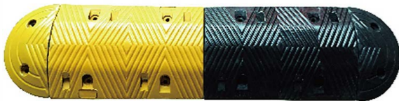
Model (型号): CC-B03 Centre Section (尺寸): 500x330x70mm End Section (端头): 170x330x70mm
