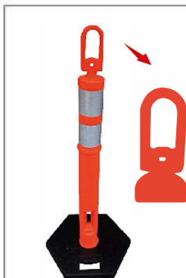
Model:CC-F07 Height:1100mm Base size:420x420mm Base weight:6kg Post weight:0.8kg PCS/M 2 :45PCS
