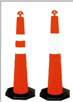
Model:CC-F02 Height:1100mm Weight(total):9kg Base size:420x420mm Base weight:8kg Post weight:1kg PCS/M 2 :55PCS
