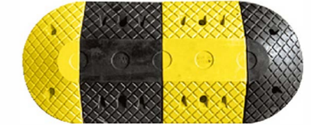
Model (型号): CC-B16 Centre Section (尺寸): 250x400x70mm End Section (端头): 200x400x70mm 1 Channel: H32xW58mm
