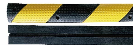
Model (型号): CC-B33 Size (尺寸): 1000 x 150 x 30mm 1 Channel: H20xW25mm
